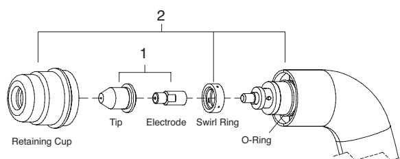
Consumable Kits for HP-50 Torch
