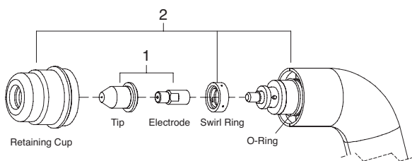
Consumable Kits for HP-70 Torch
