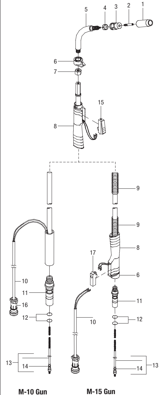
M-10 Gun
